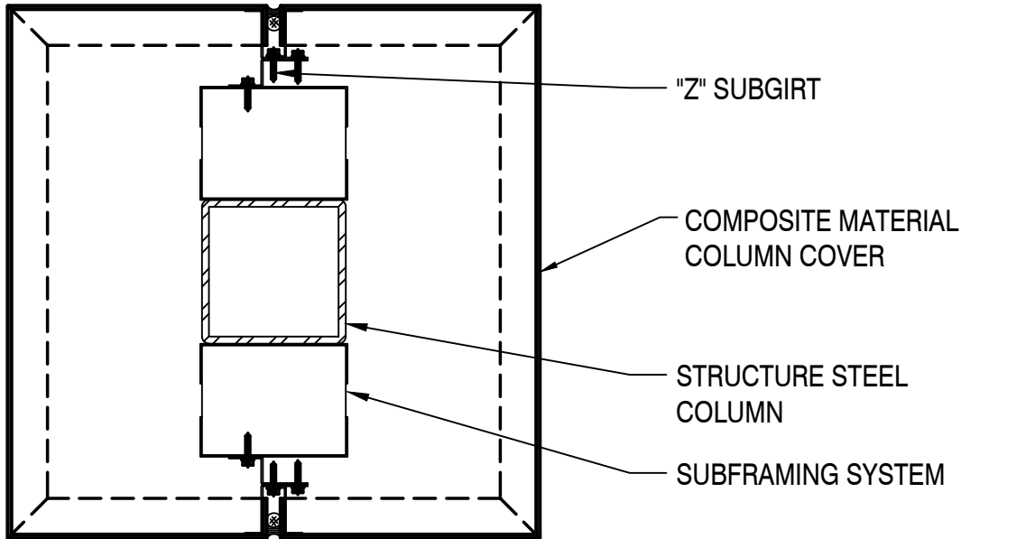
SECTION A
